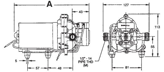
A = 197mm for 7 ltr models, A = 226mm for 10 ltr models. Approximate measurements for all pumps
