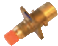
GT622 Remote Electronic tank level indicator. 12 volt only
