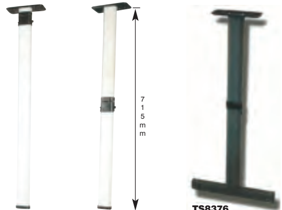
TS8050 TS8350 LIGHTWEIGHT FOLDING TABLE LEGS
