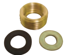
Reducing collar 1/2" BSP male x 3/8" BSP female. DLTRF0538 Reducer
